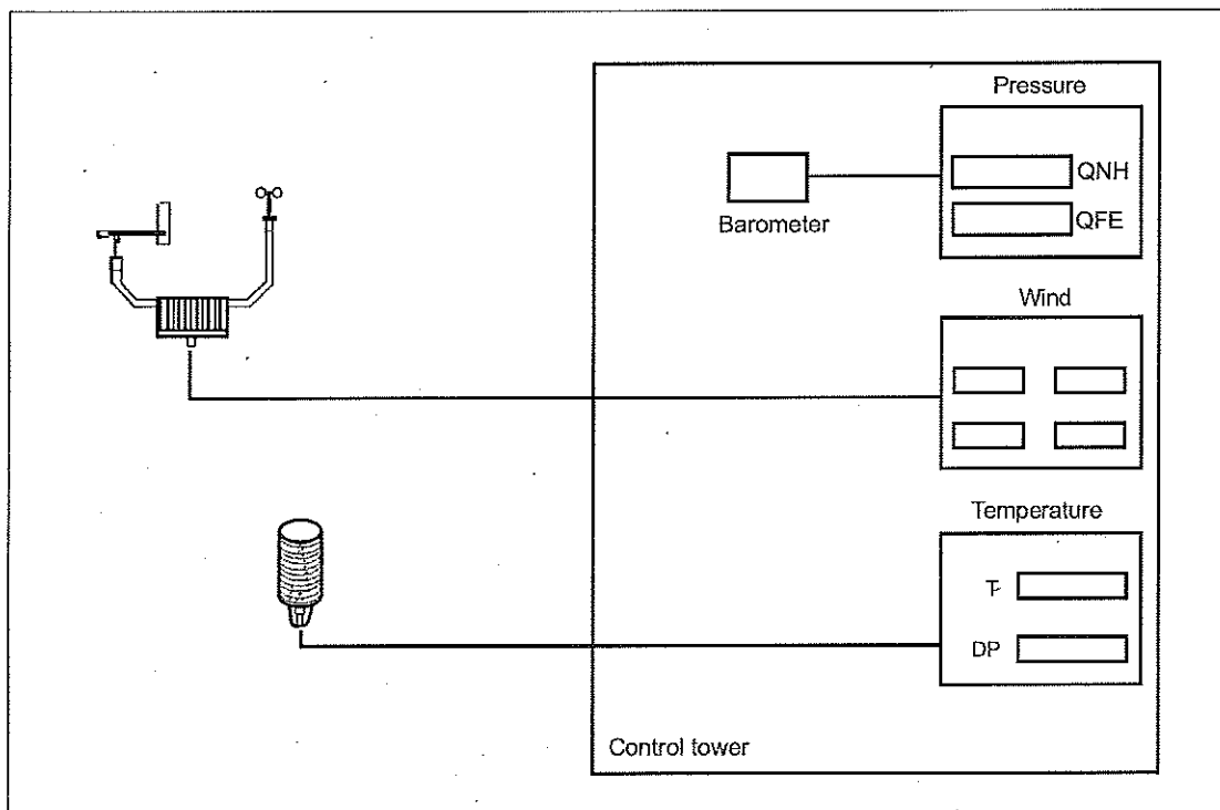
Figure 11-3. Simple system with pressure, temperature, wind sensors and dedicated displays
