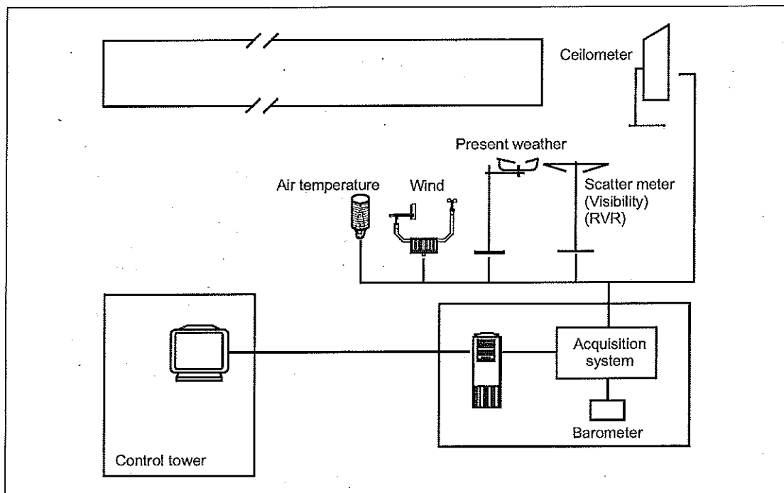
Figure 11-2. ASOS-type automatic system, with wind, temperature, pressure, scatter metre, ceilometer and present weather
